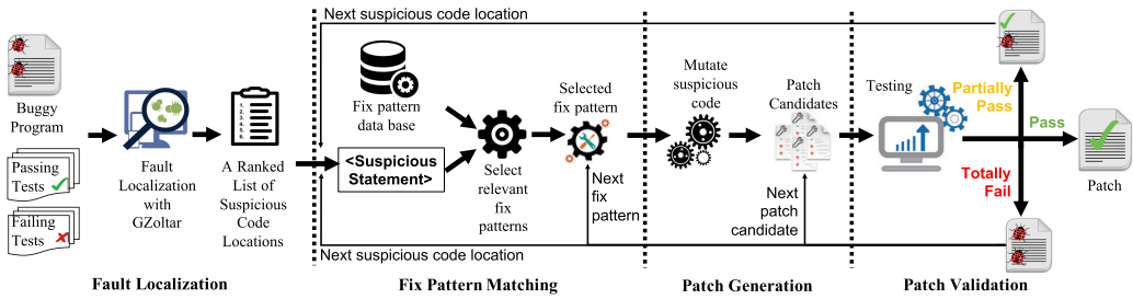
Fig. 5. Overview bug-fixing process with AVATAR.
