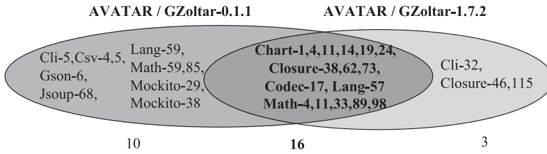
Fig. 21. Bugs correctly fixed by AVATAR under GZoltar 0.1.1 and 1.7.2, respectively.
