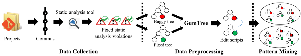
Fig. 2. Summarized steps of static analysis violation fix pattern mining.
