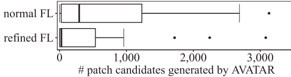
Fig. 26. Comparison on the number of patch candidates generated by AVATAR with normal and refined FL.
