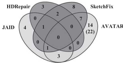
Fig. 19. Relationship of correctly fixed bugs by HDRepair, JAID, SketchFix, and AVATAR, respectively.
